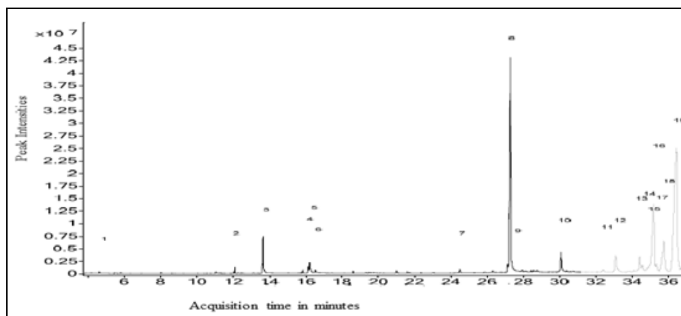
FIG. 1: GC-MS CHROMATOGRAM OF ETHYL ACETATE EXTRACTS OF L. CORNUTA
