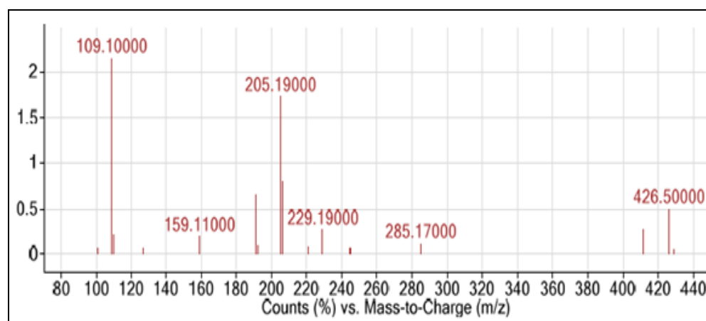
FIG. 2: THE MASS SPECTRUM OF THE UNKNOWN COMPOUND NUMBER 13ELUTING AT 34.9 MINUTES. THE MOST ABUNDANT MOLECULAR IONS FOR THE COMPOUND ARE 109.1 FOLLOWED BY 205.19 AND THE MOLECULAR ION IS 426.5
