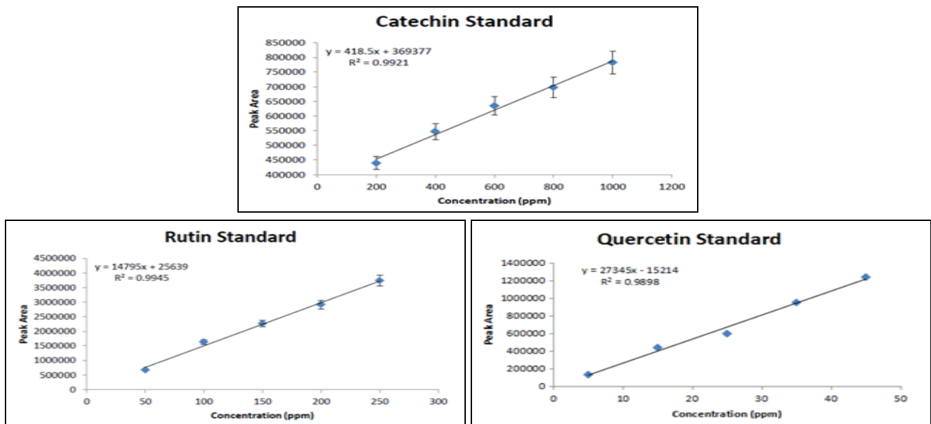
FIG. 3: HPLC STANDARD CURVES
