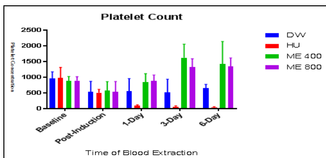
FIG. 1: MEAN PLATELET COUNT ( \times 10^9 PER LITER)
