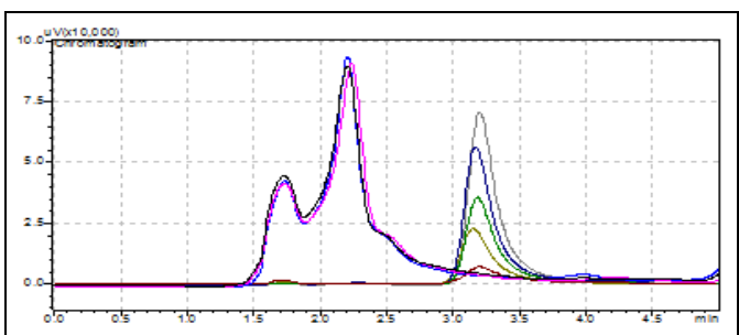
FIG. 6: OVERLAY OF STANDARD QUERCETIN AND PLANT SAMPLE
