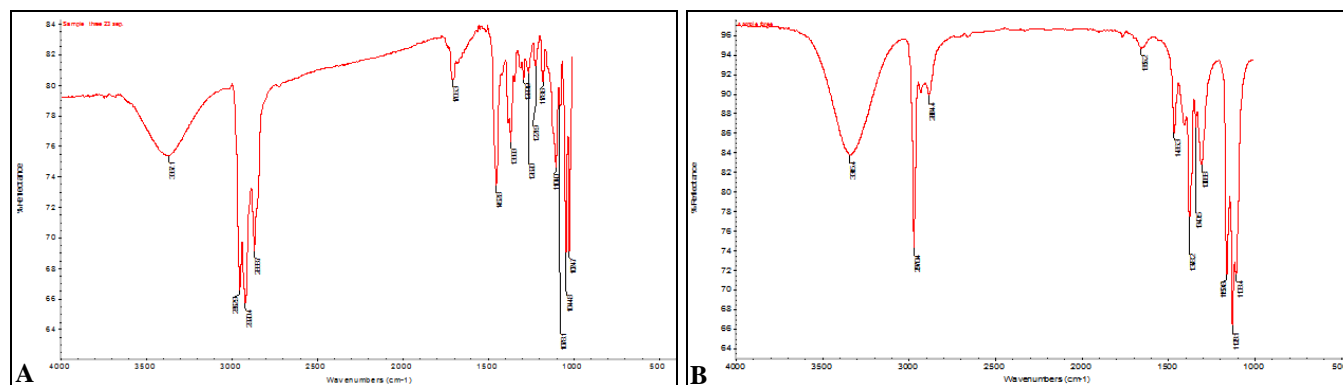
FIG. 1: FT-IR SPECTRA OF ESSENTIAL OILS EXTRACTED FROM MENTHA PIPERATA (1A) AND MENTHA ARVENSIS (1B) USING ATTENUATED TOTAL REFLECTANCE MODE
