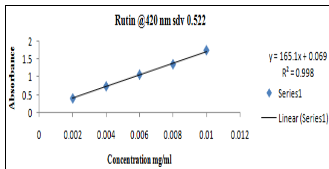
FIG. 9: CALIBRATION CURVE
