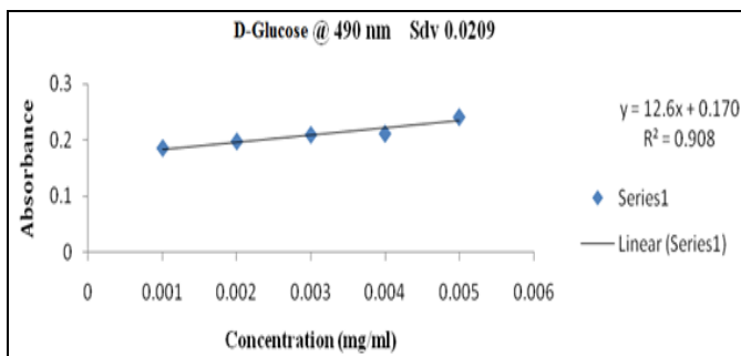
FIG. 6: CALIBRATION CURVE
