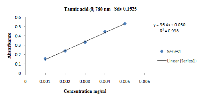
FIG. 7: CALIBRATION CURVE
