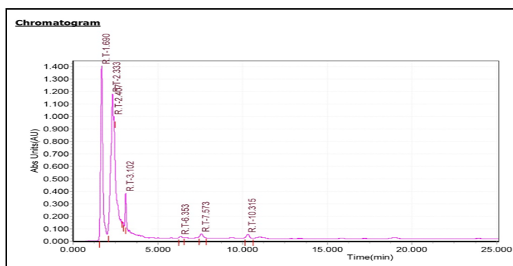
FIG. 1: HPLC PEAKS
